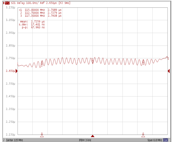
Group Delay Variation Fo \pm 2.3\text{MHz}
