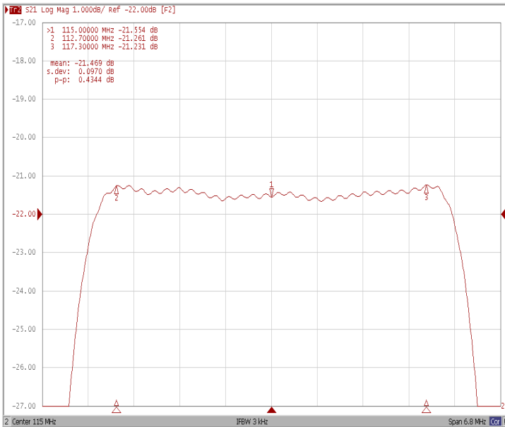
Ripple Variation Fo \pm 2.3\text{MHz}
